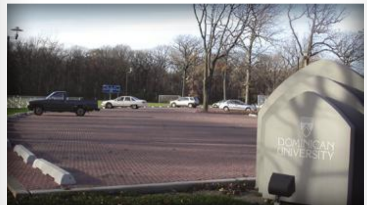
PICP lot eliminates need for detention basin at Dominican University, Chicago.
